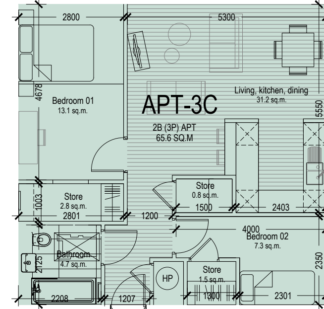
Apartment Type 3C Area - 65.6 SQM Apartment blocks 3 & 4
