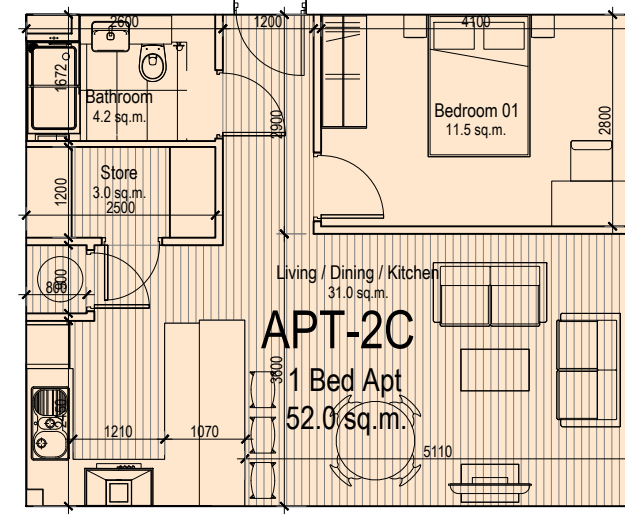
Apartment Type 2C Area - 50.0 SQM Apartment blocks 1 & 2
