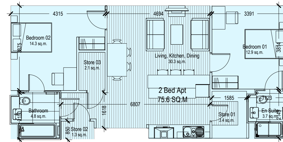
Apartment Type 4D Area - 75.6 SQM Apartment blocks 3, 4 & 5
