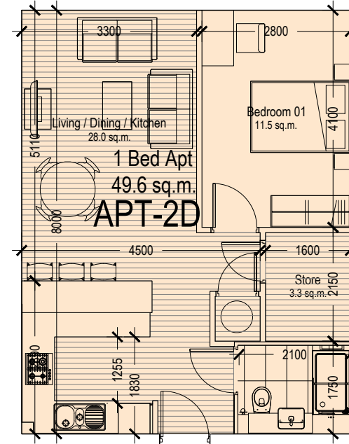
Apartment Type 2D Area - 49.6 SQM Apartment blocks 3, 4 & 5
