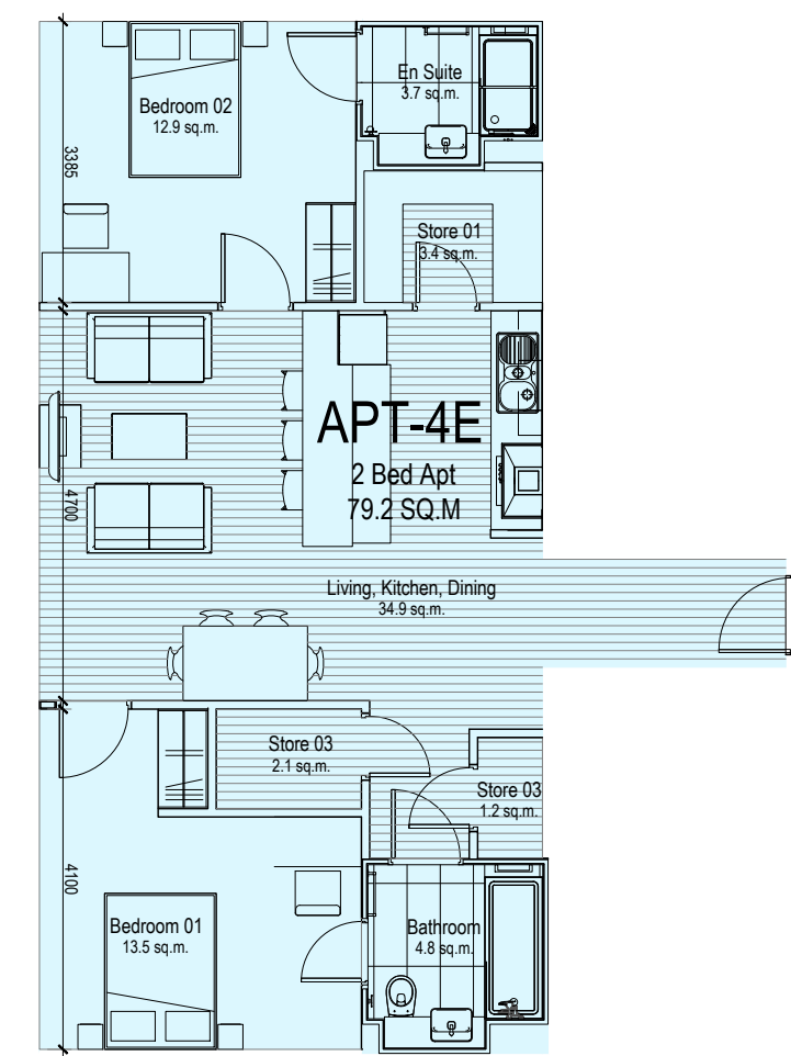
Apartment Type 4E Area - 79.2 SQM Apartment blocks 5
