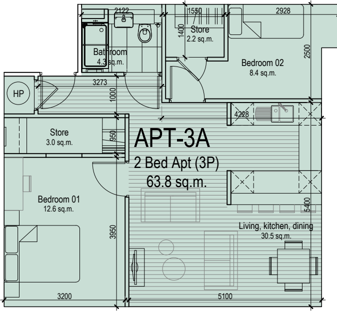
Apartment Type 3A Area - 63.8 SQM Apartment blocks 1 & 2
