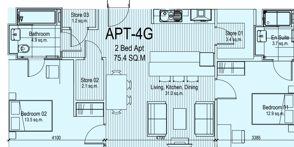
Apartment Type 4G Area - 75.4 SQM Apartment blocks 5
