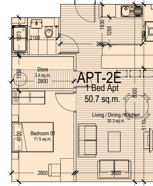
Apartment Type 2E Area - 50.7 SQM Apartment blocks 3 & 4
