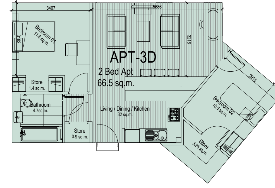
Apartment Type 3D Area - 66.5 SQM Apartment blocks 5
