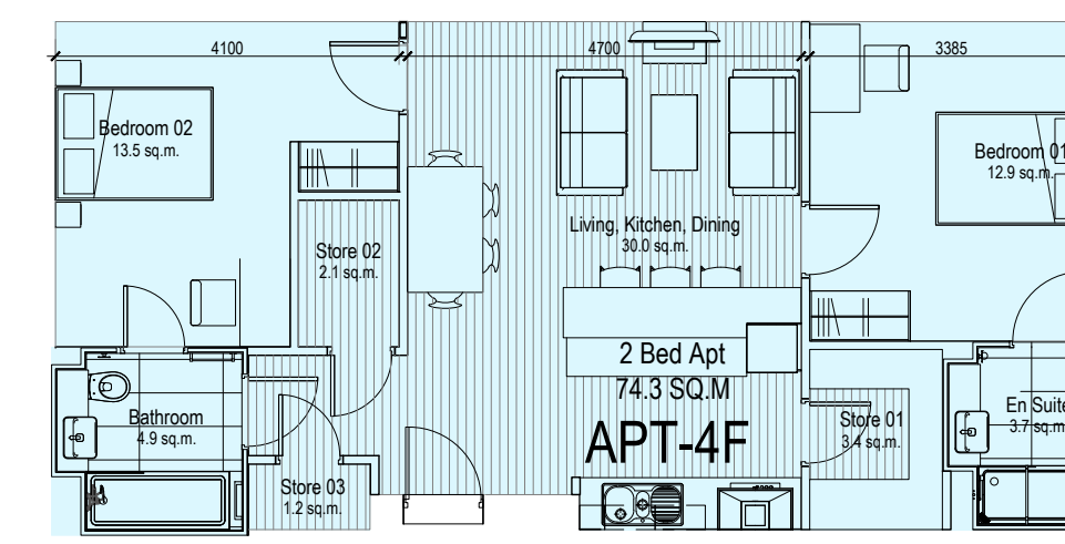
Apartment Type 4F Area - 74.3 SQM Apartment blocks 5
