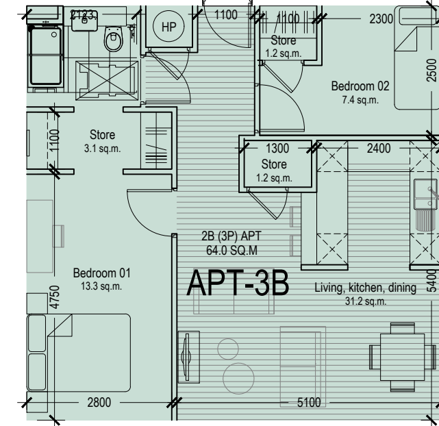
Apartment Type 3B Area - 64.0 SQM Apartment blocks 1 & 2
