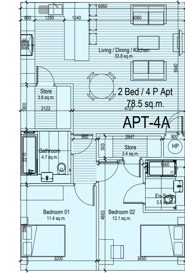
Apartment Type 4A Area - 78.5 SQM Apartment blocks 1 & 2
